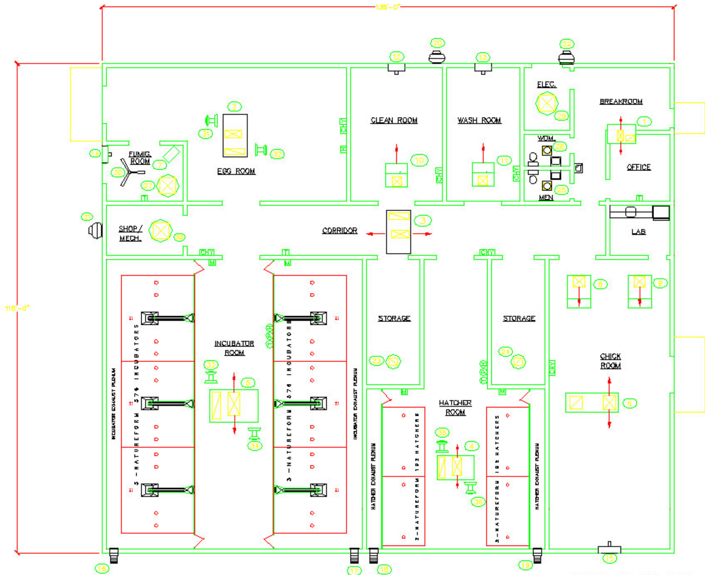
FLOOR PLAN FOR (6) NATUREFORM 576 SETTERS AND (4) 192 HATCHERS
